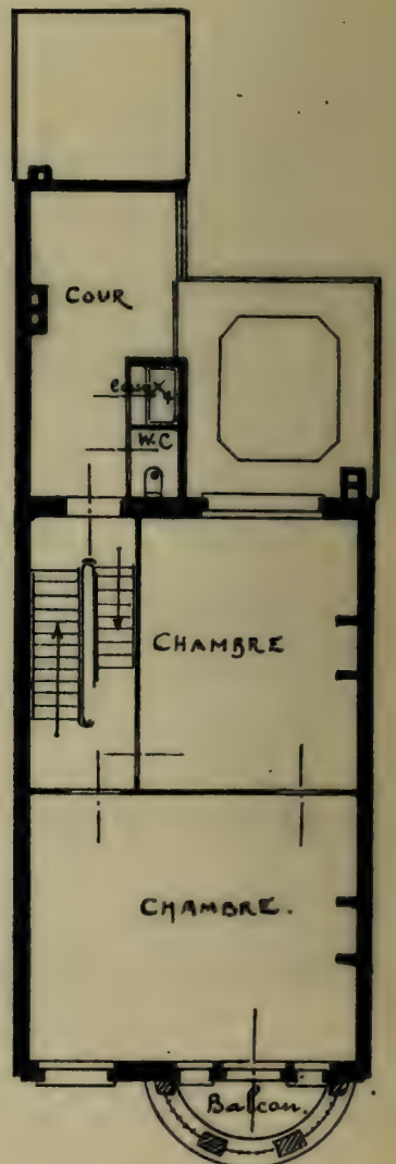
SECOND ETAGE.
